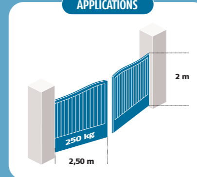
Axovia 170S NS can be fitted to any metal swinging gates, new or existing.
