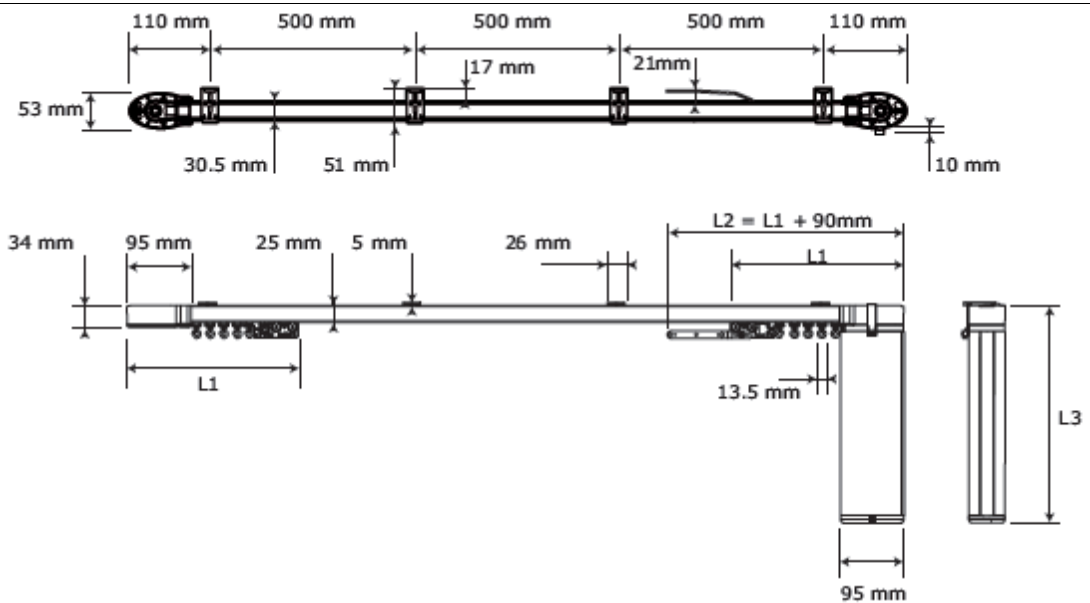
Dimensions for Central Opening Pinch Pleat. S-Fold and Heavy Duty Options also available
